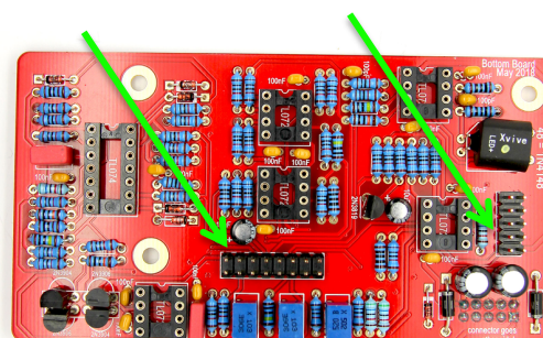
Bottom Board
